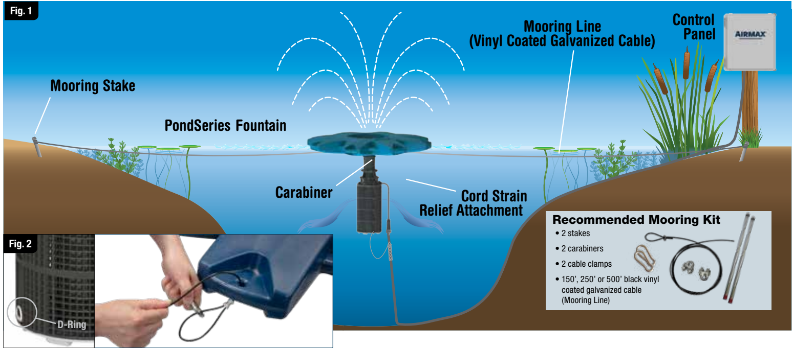
Strain Relief
