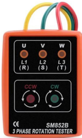
3-Phase Sequence Rotation Tester (Airmax Item # 650941)
